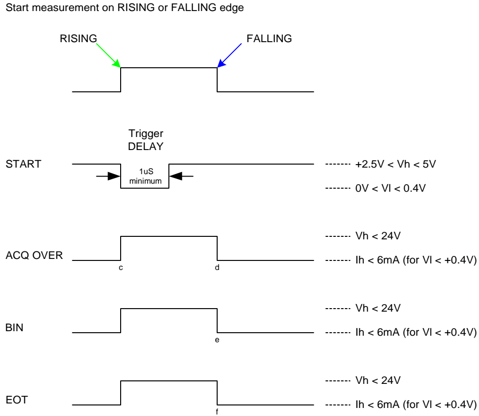
Figure 3-6: Trigger
