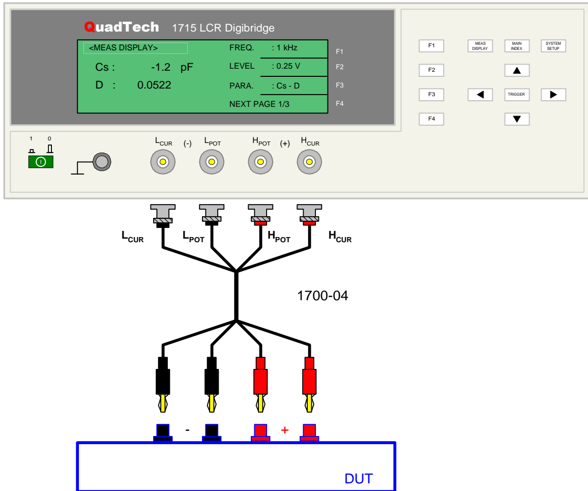
Figure 2-12: 1700-04 BNC/Banana Plug Test Lead Set
