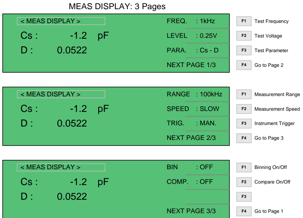
Figure 2.2: MEAS DISPLAY
