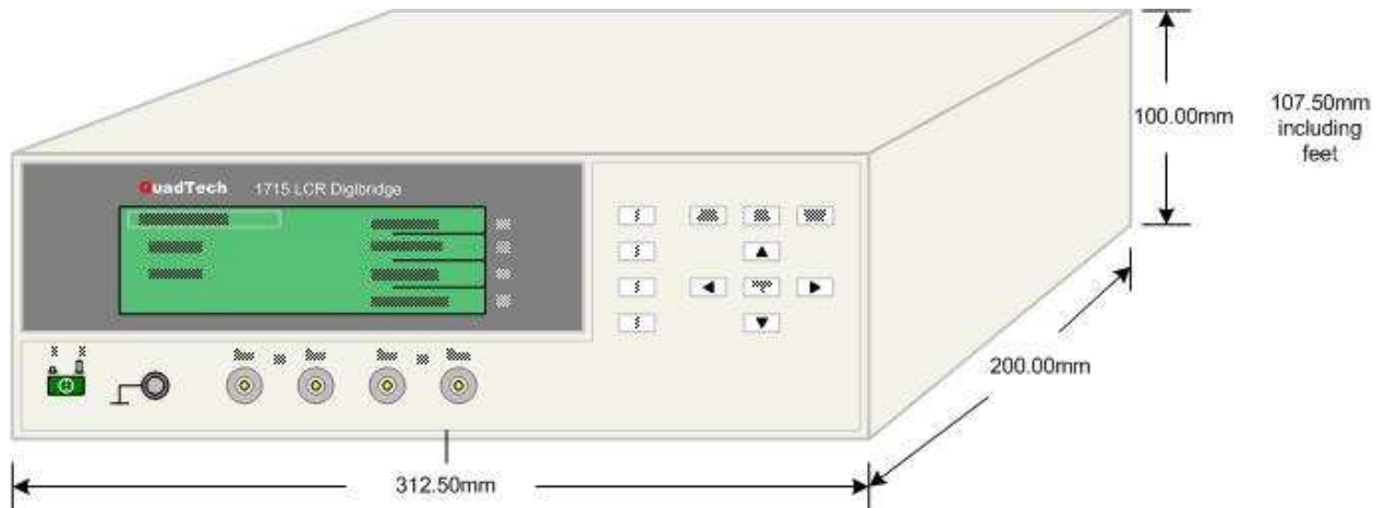
Figure 1-4: 1715 Instrument Dimensions
